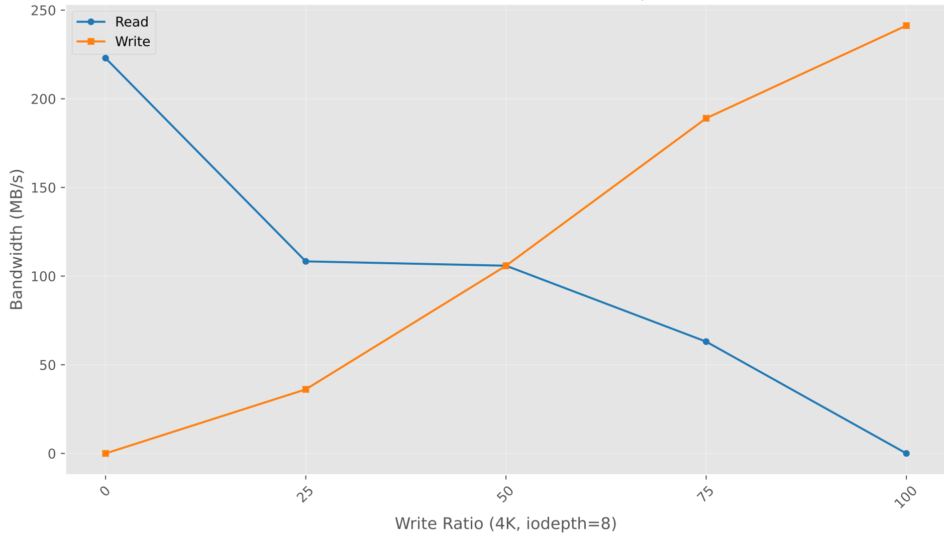
Bandwidth vs Write Ratio (4K, iodepth=8)
